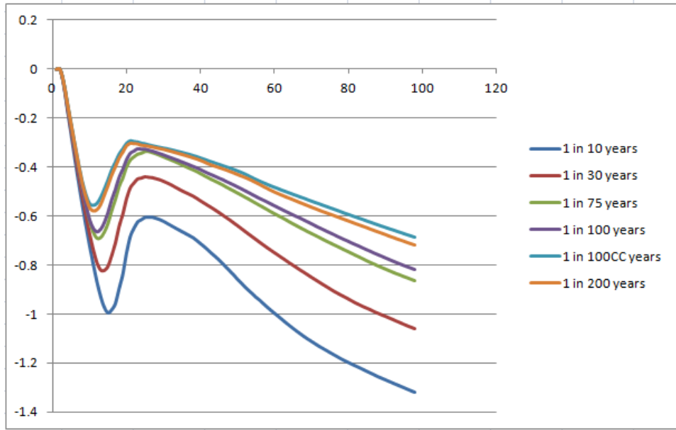
Figure 6-1: Mass Balance
