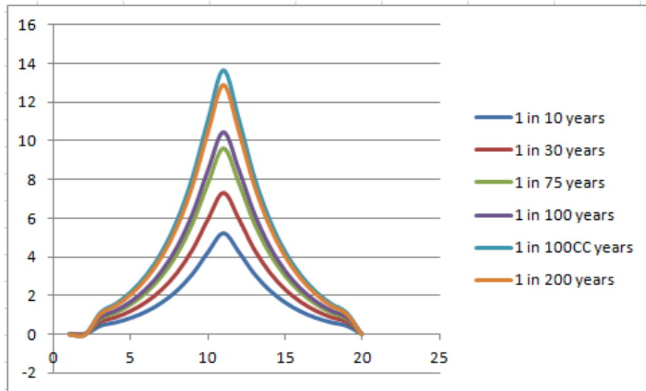
Figure 3-2: Rainfall Hyetographs
